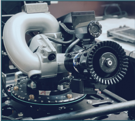
WATER/FOAM CANNON
